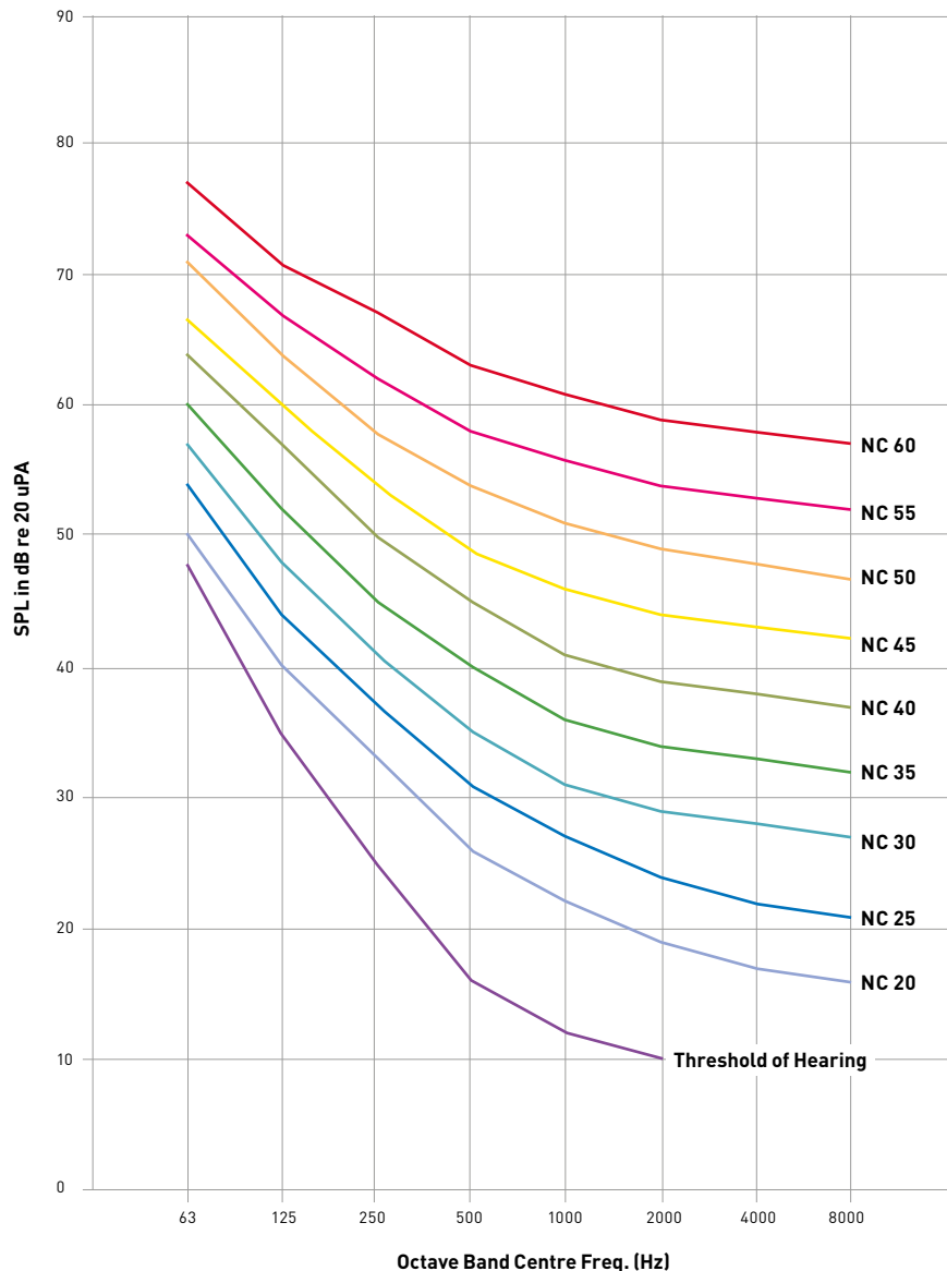
Noise Criteria (NC) Curve
