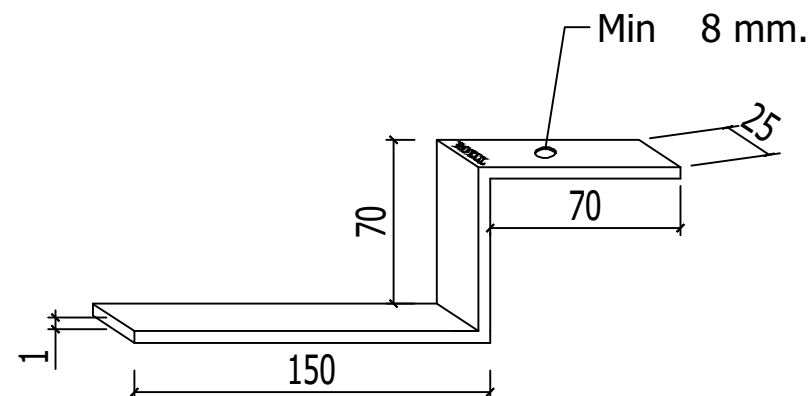
Galvanized steel fixing Z-brackets Detail A
