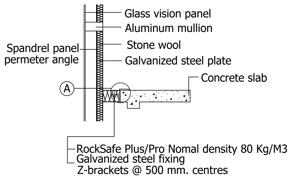
SECTIONAL VIEW
