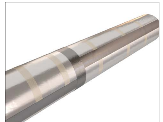
Figure 10: Application of vapour barrier tape on a circumferential joint
