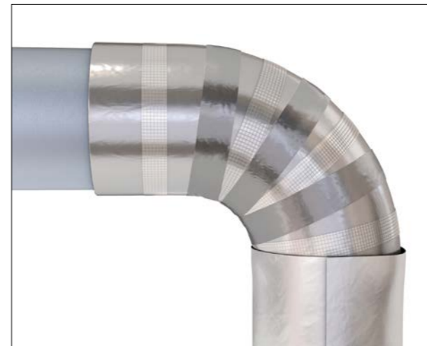
Figure 66: Secure overlap with roller
