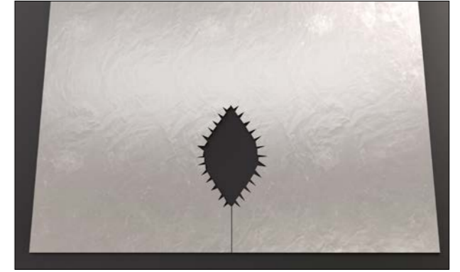
Figure 71: Template of primary vapour barrier for equal tee
