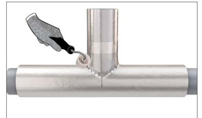
Figure 73: Securing joints with roller
