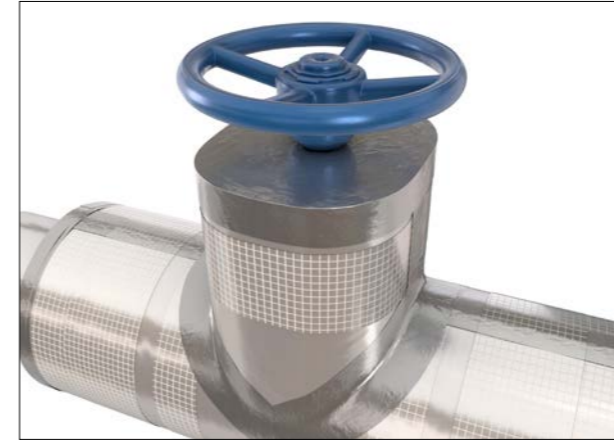
Figure 51: Application of vapour barrier tape at all joints and seams
